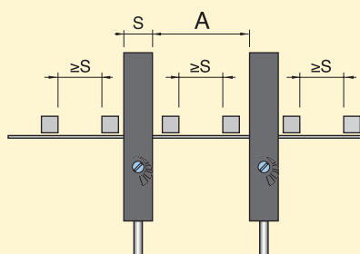
DISTANZA FRONTALE / FRONT DISTANCE
