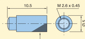
LENTE MOD. AT 4101 - ACF000006 LENS VIEWER AT 4101
