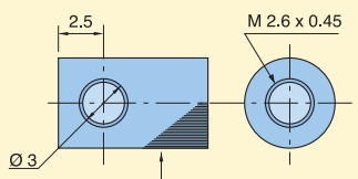
DEVIARAGGIO MOD. AT 4102 - ACF000007 LENS VIEWER 90° AT 4102
