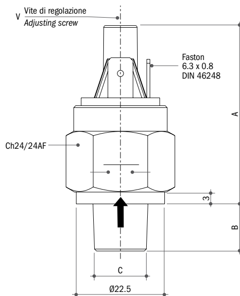
Contatto NC NC contact
