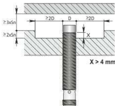
Non flush mounting
