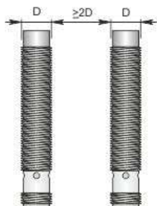
Side by side mounting
