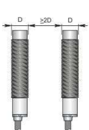
Side by side mounting
