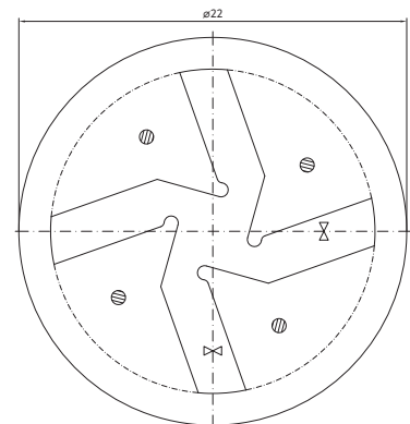
Profile cross-section Quadro-Profile 3100.8000F
